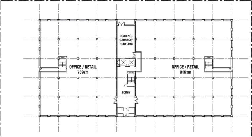
Ground Level
